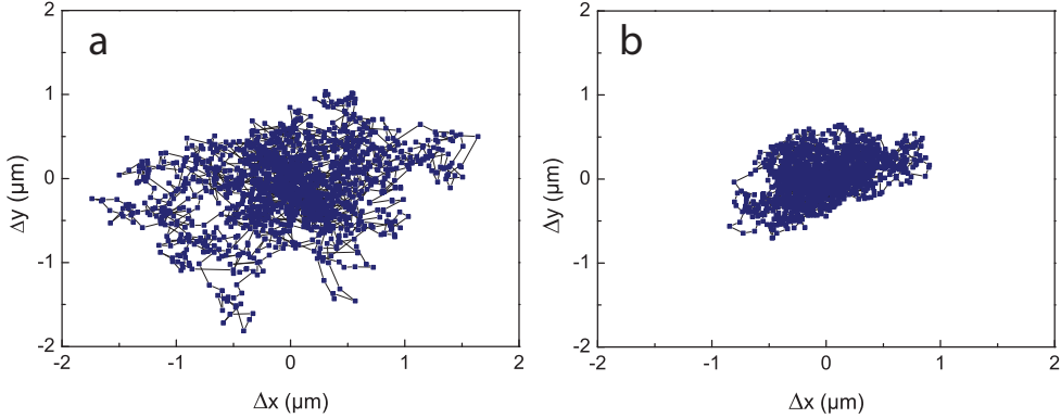
Figure 3.7: \Delta x - \Delta y trajectories recorded during the same time interval \Delta t = 55 \text{ s} of two spheroids with different aspect ratios: \phi = 1.4 (a) and \phi = 8.7 (b).
