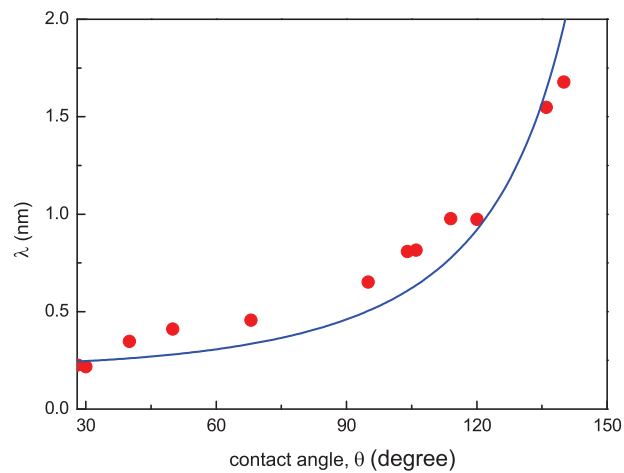
Figure 4.20: Points: lateral correlation length \lambda of the capillary waves, here used as free parameter, as a function of the contact angle \theta . Values of \lambda are computed according to eq. 4.72 in order to recover the measured additional drag (see fig. 4.19). Solid line: the behavior \lambda \sim 1/(1 + \cos \theta) is proposed to fit the experimental data (eq. 4.75).
