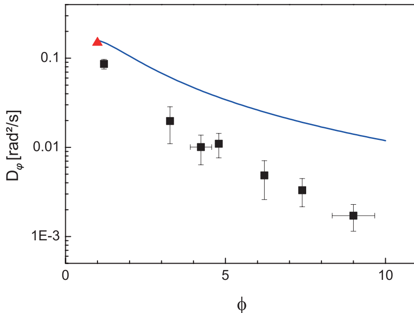
Figure 3.19: Rotational diffusion coefficient D_\phi vs. aspect ratio \phi in semi-log scale. Points are direct measurements of the rotational diffusion coefficient, averaged on the values on 3 to 6 particles. Error bars are the standard deviation of the average. At \phi \simeq 1 the trend of the curve recovers the value for the optically anisotropic Janus particle (red point). When the aspect ratio increases, the rotational diffusion coefficient varies over 2 decades. This behavior differs from the one predicted when the particle is immersed in water (solid line).
