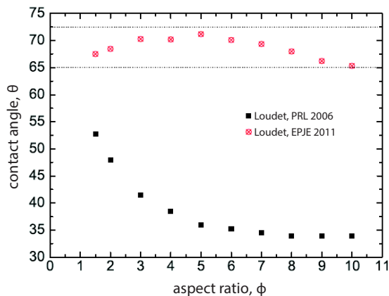
Figure 1.17: Contact angle \theta as a function of the aspect ratio \phi , obtained via PSI measurements of the distortion \Delta h and numerical solution of the interfacial profile. Since \Delta h is a non-monotonous function, two possible branches for \theta are derived. Image from Loudet and Pouligny, EPJE 34, 76 (2011) [41].
