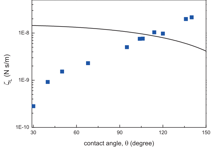
Figure 4.14: Points: additional drag \zeta_L versus contact angle \theta , in a semi-log scale. The values are recovered from experimental drag measurements (fig. 2.12), according to eq. 4.44. Solid line: hydrodynamics drag at the interface \zeta_H versus \theta , computed from the model provided by Fischer et al. [29]. \zeta_L is negligible for small contact angles ( 30^\circ - 60^\circ ), but it is comparable to, and also overcomes, the hydrodynamics drag for \theta > 90^\circ .
