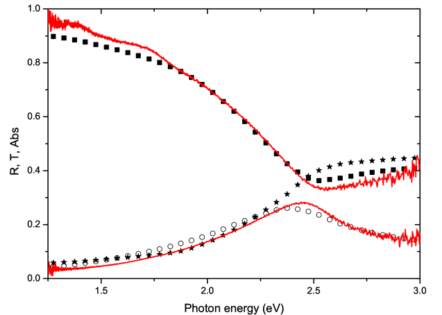
FIG. 1: Transmission (open circles), reflection (black squares) and absorption (stars) of a layered structure consisting of a 28 nm thick gold buffer layer, 6 monolayers of cobalt and 15 monolayers of gold on a glass substrate, computed from the effective medium model using dielectric constants from Ref. [16, 17, 19]. Light scattering has been neglected. Full red line : experimental reflection and transmission coefficients normalized to the values computed at 2.35 eV
