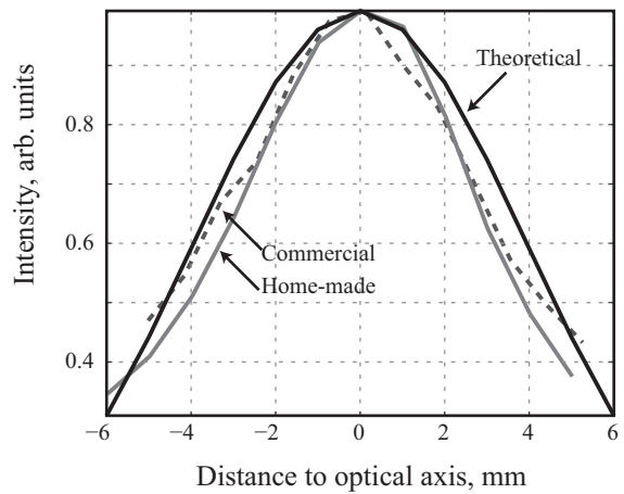
Fig. 3. Horn characterization at 290 GHz. The top graph represents the far-field intensity measured in a plane orthogonal to the optical axis for the home-made horn. The bottom graph presents a cut of the intensity along the x direction for the home-made horn and the commercial horn. The theoretical intensity is calculated using a Gaussian-beam propagation simulation.
