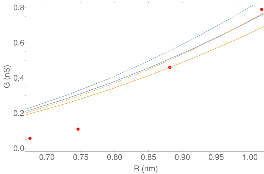
Figure 4. Fit of the conductance simulation data (red dots) for CNTs of length L=10 nm and various radii with the TIP3P water model. The blue (respectively orange) curve corresponds to a fit of the two last (reps. four) points. The dashed curves correspond to the case without access resistance.
