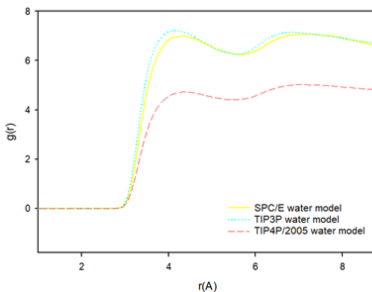
Figure 6. Radial density distribution of water oxygen atoms towards carbon atoms within (13,13) CNT (cyan dotted points, yellow and red dotted curves represent TIP3P, SPC/E and TIP4P/2005 water models).
