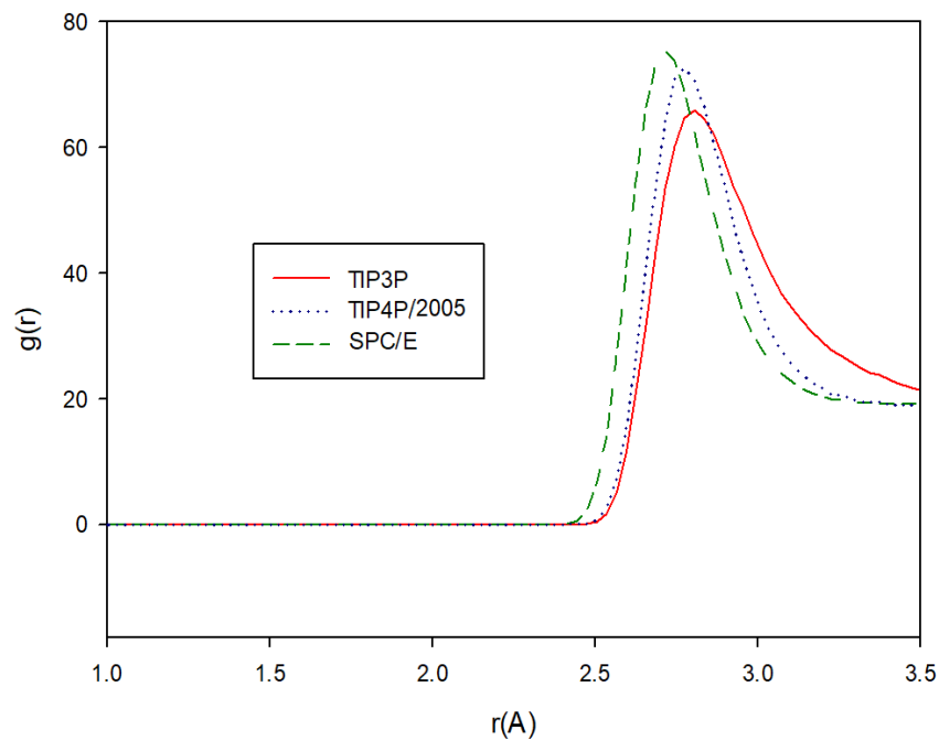
Figure 7. Radial density distribution of water oxygen atoms within (13,13) CNT (green, blue and red dotted curves represent SPC/E, TIP4P/2005 and TIP3P water models, respectively).
