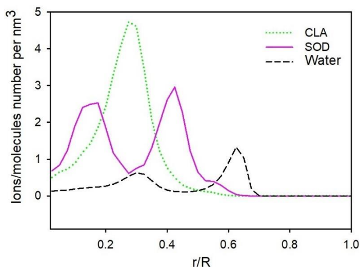
Figure 8. Water and ions distribution inside (13,13) CNT (Cl - ions are in green dotted lines; Na + in pink and water in black dashed lines). Results obtained for a) TIP3P, b) SPC/E and c) TIP4P/2005 models, respectively.
