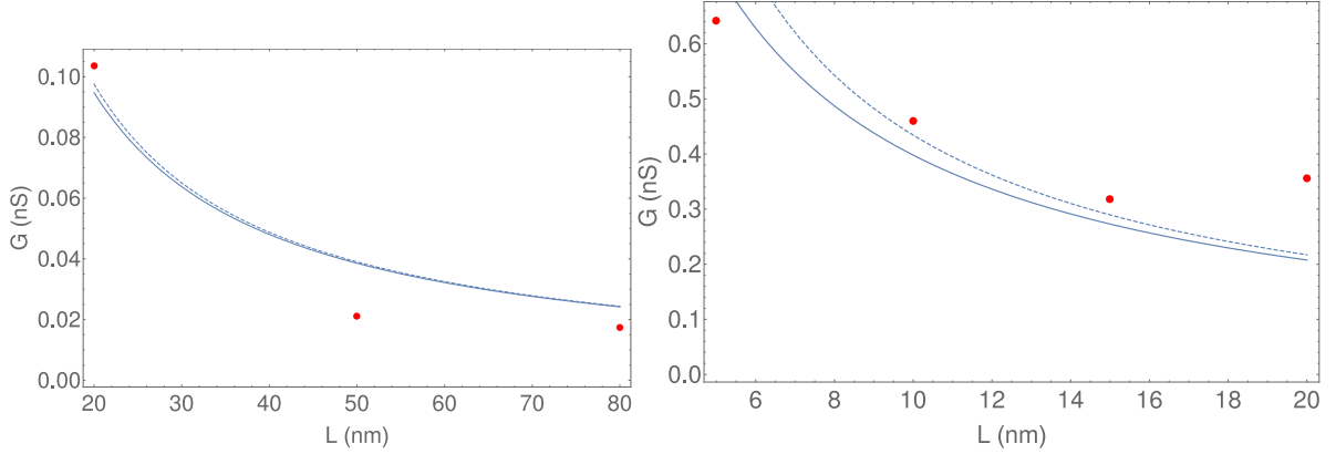
Figure 10. Fit of the conductance simulation data (red dots) for the (10,10) (left) and (13,13) (right) CNTs vs. their length L with the TIP3P water model. Blue solid curves correspond to a fit with Eq. (1), dashed ones corresponds to the case without access resistance.
